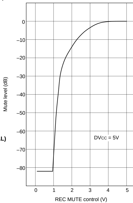
REC MUTE characteristics
