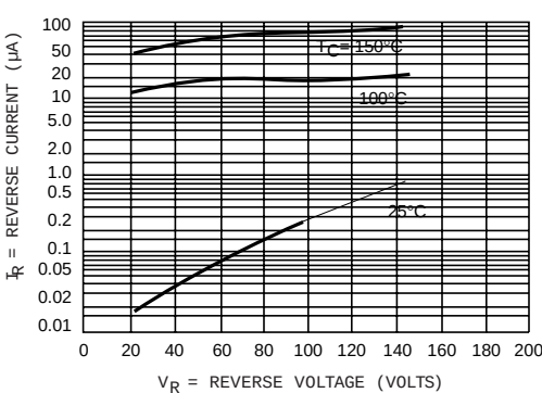
TYPICAL REVERSE CURRENT 1N6768, 1N6769, 1N6770, 1N6771
