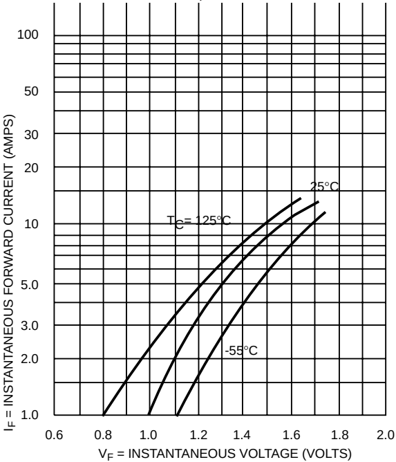
TYPICAL FORWARD VOLTAGE 1N6772, 1N6773
