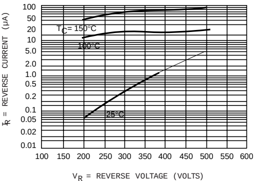
TYPICAL REVERSE CURRENT 1N6772, 1N6773
