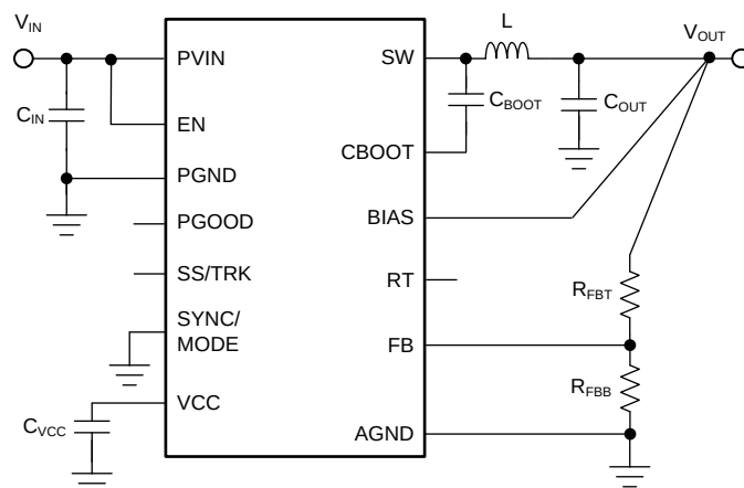
图 25. LM73605/6 Basic Schematic
