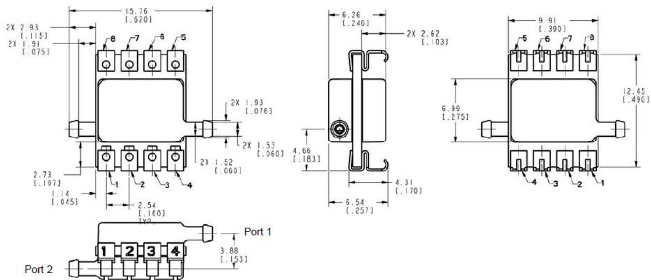
Figure 4. Package Dimensional Drawings (continued)
