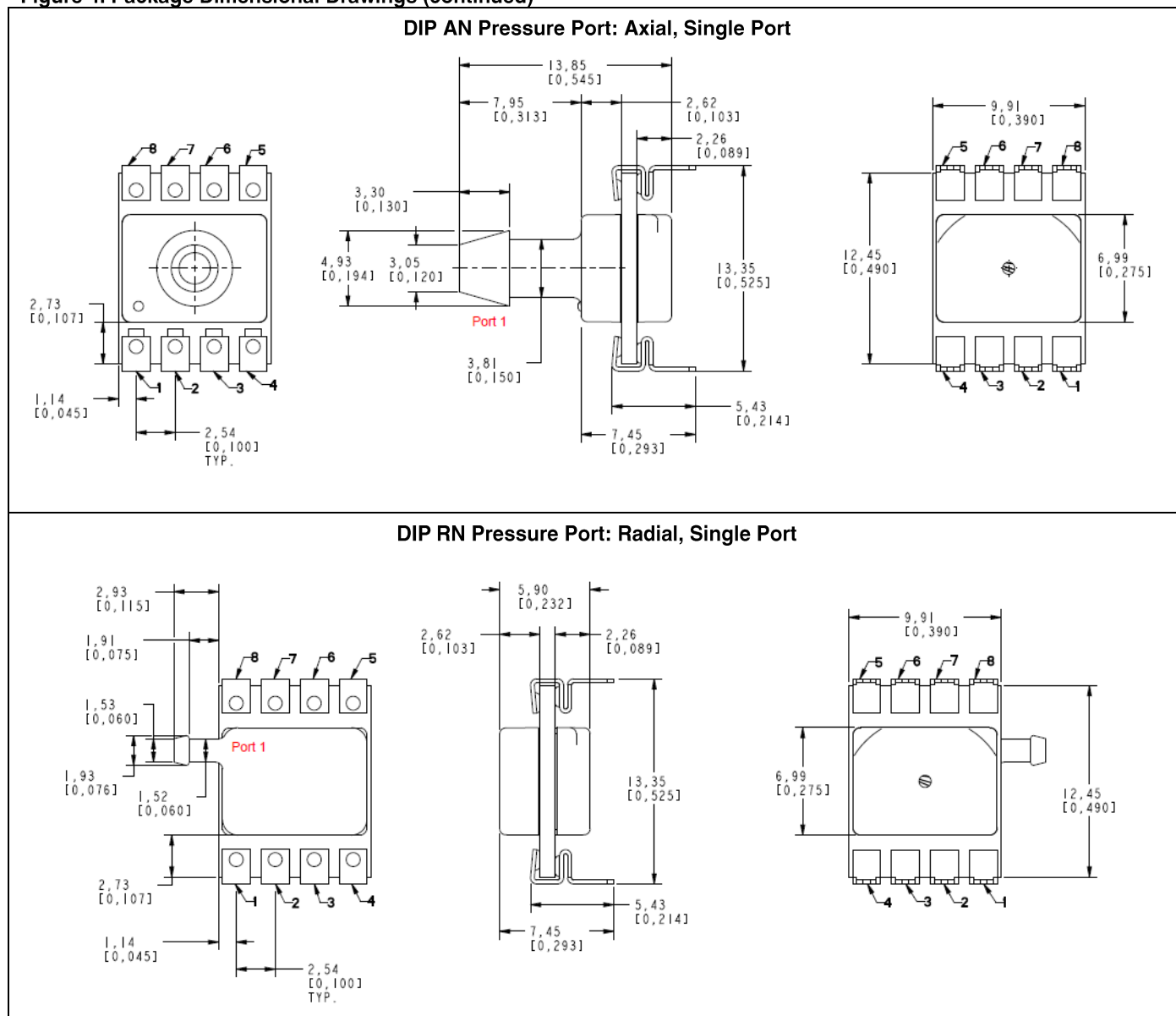
Figure 4. Package Dimensional Drawings (continued)
