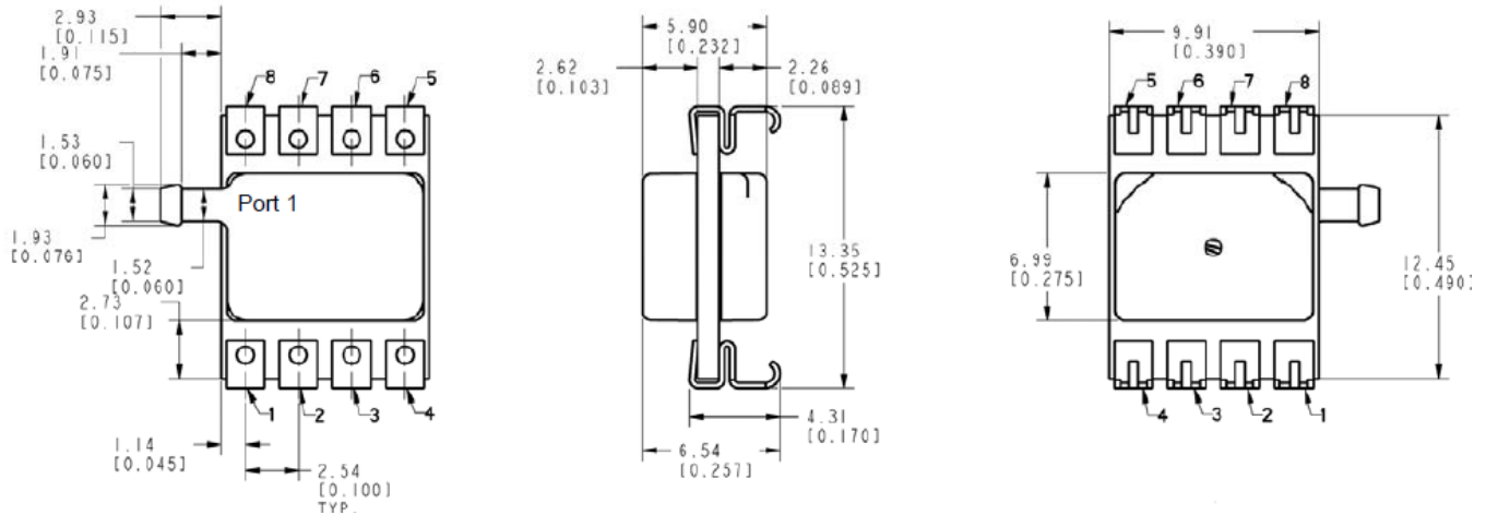
SMT RR Pressure Port: Radial, Dual Ports on Same Side
