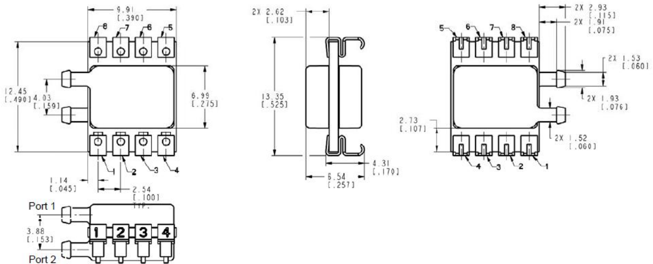
SMT RR Pressure Port: Radial, Dual Ports on Same Side
