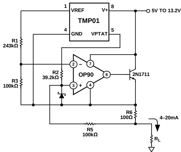
Figure 27. 4mA to 20mA Current Loop
