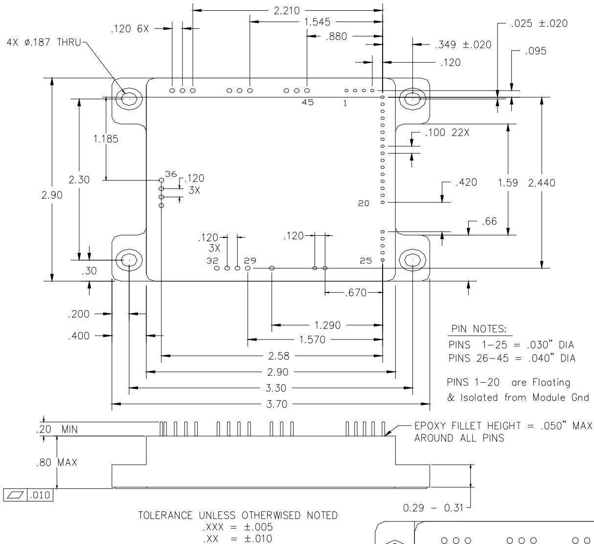
Figure 2. Mechanical Outline
