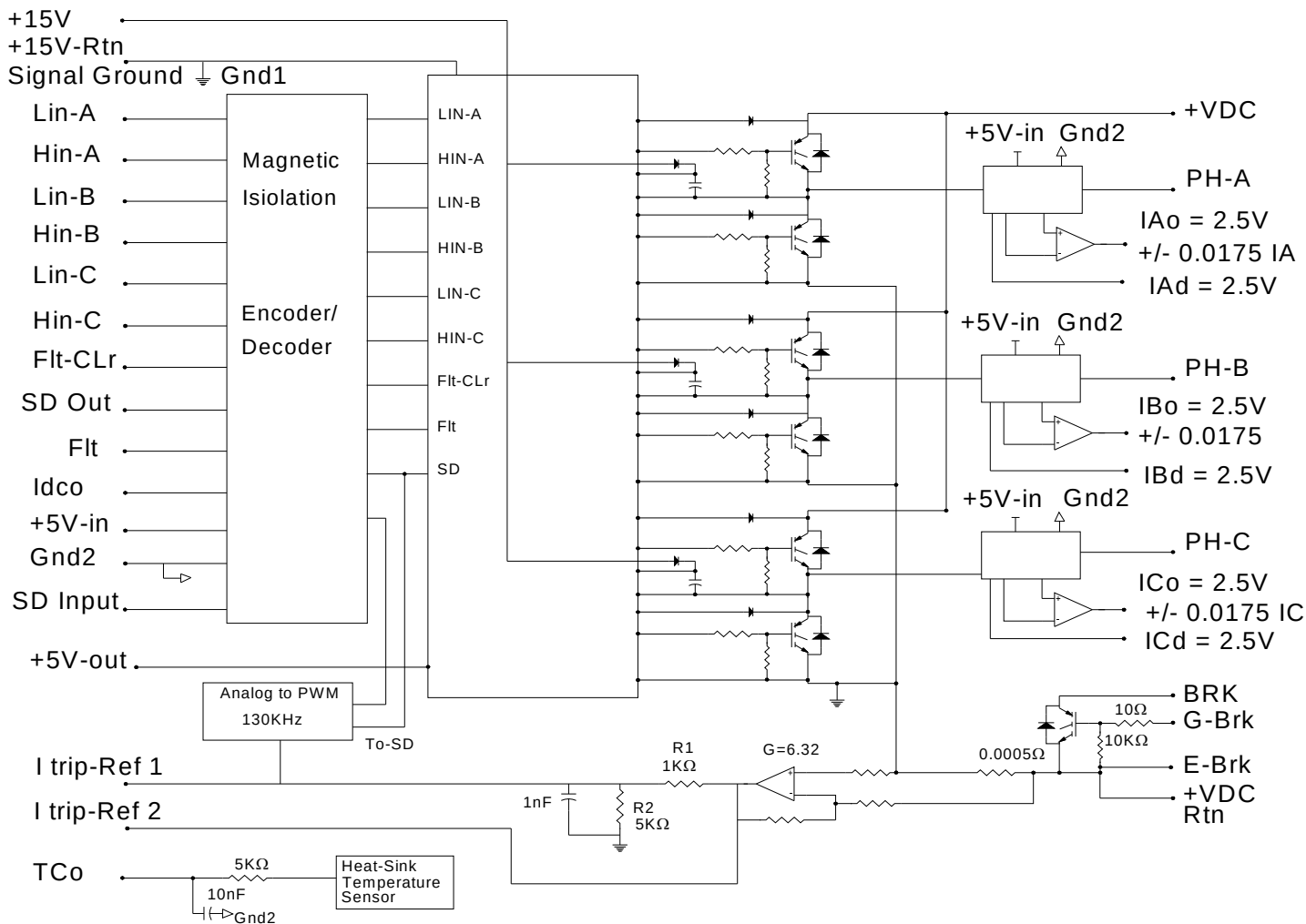
Fig. 1. Block Diagram
