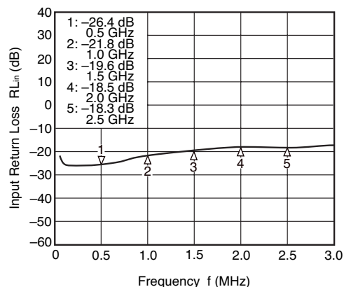
INPUT-OUTPUT2 INPUT RETURN LOSS vs. FREQUENCY
