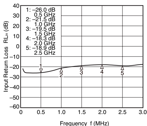
INPUT-OUTPUT1 INPUT RETURN LOSS vs. FREQUENCY
