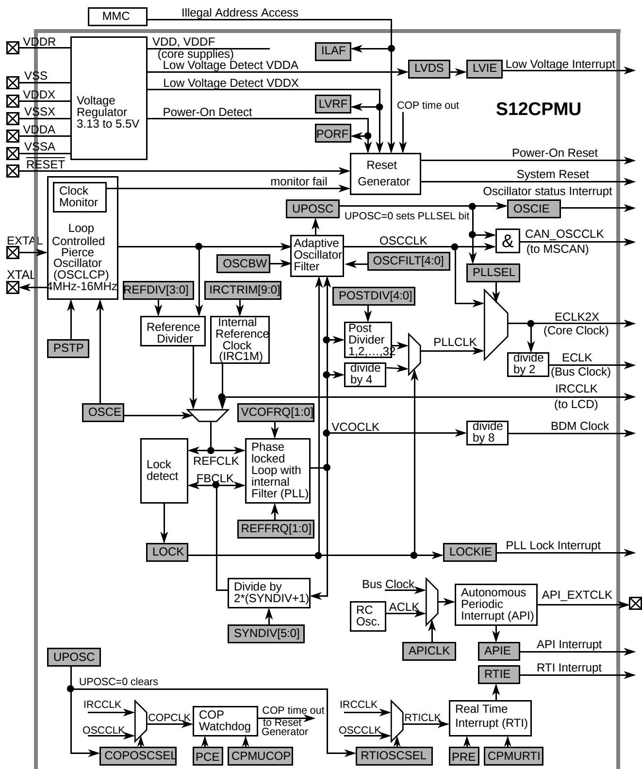
Figure 85. Block diagram of S12CPMU
