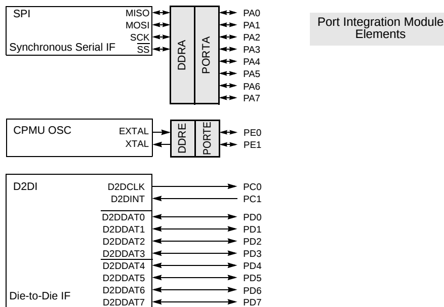
Figure 42. Block Diagram
