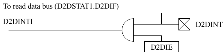
Figure 120. D2D External Interrupt Scheme
