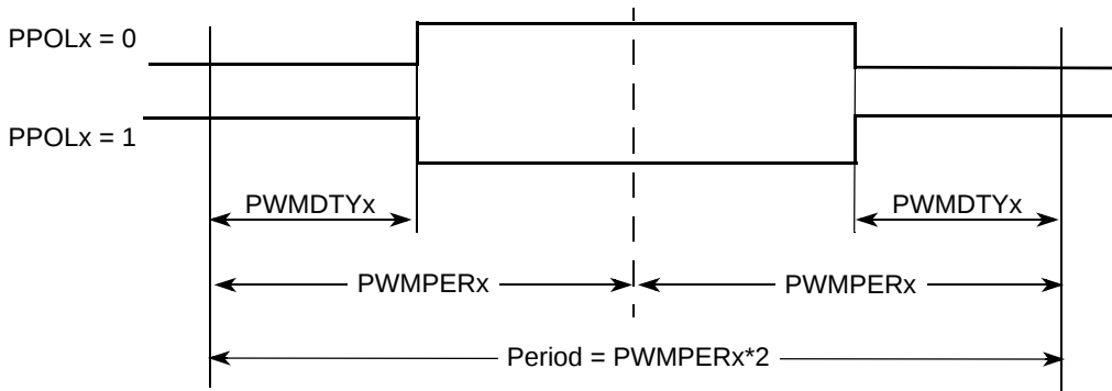
Figure 27. PWM Center Aligned Output Waveform
