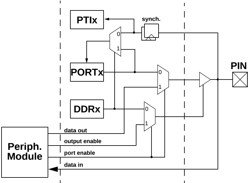
Figure 46. Illustration of I/O Pin Functionality
