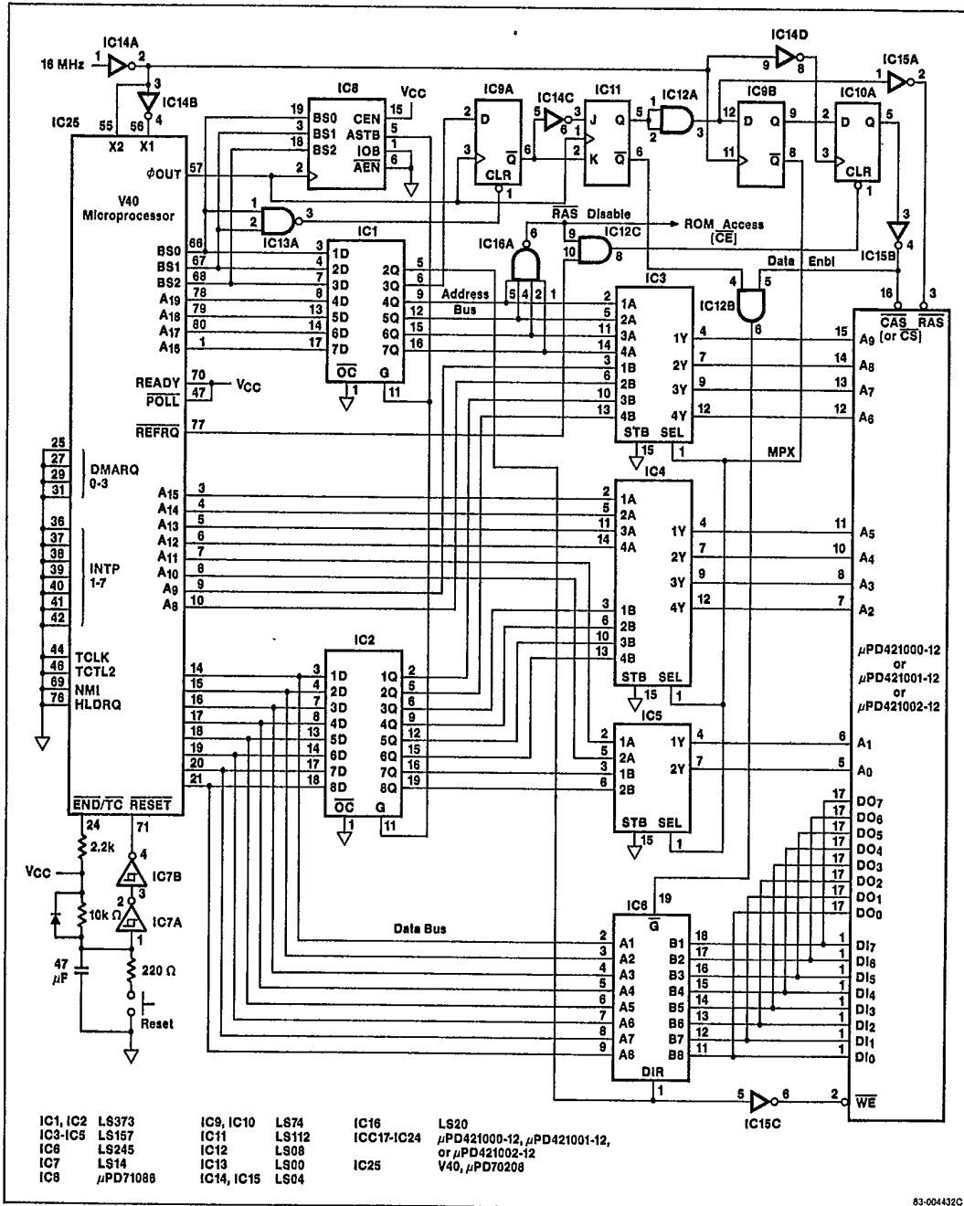
Figure 32. Composite Schematic
