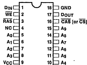
Figure 1. Pin Layouts
