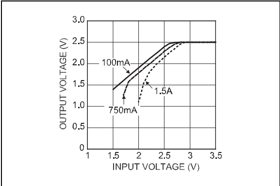
FIGURE 2-5: Dropout Characteristics.
