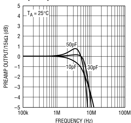
Preamp Frequency Response vs Input Capacitance
