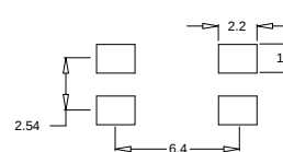
Recommended pad layout
