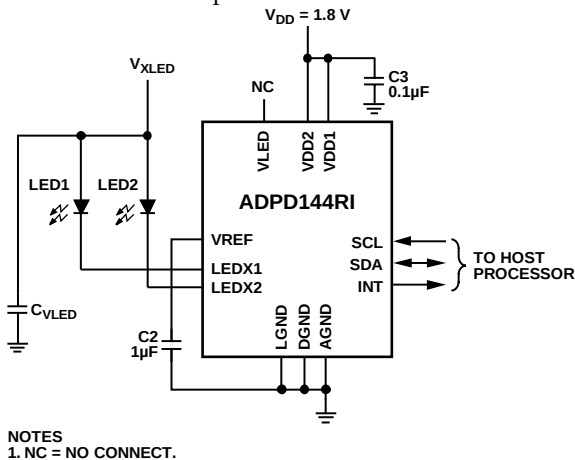
Figure 17. Connection of External LEDs
