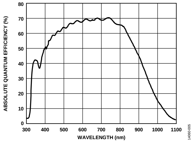
Figure 5. Photodiode Quantum Efficiency
