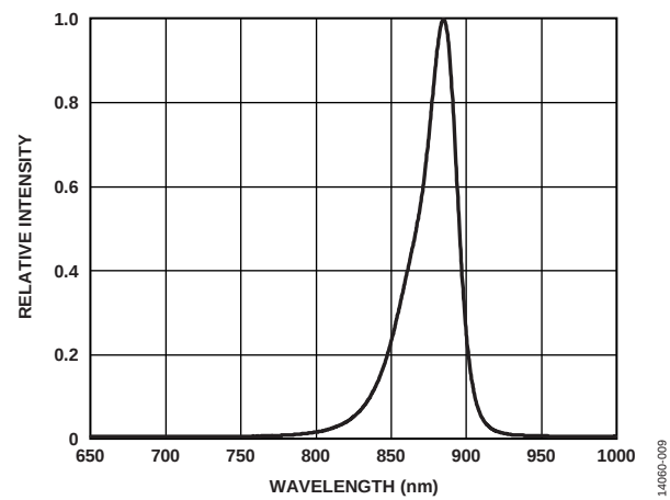
Figure 9. Spectral Output of LED2 (880 nm LED)
