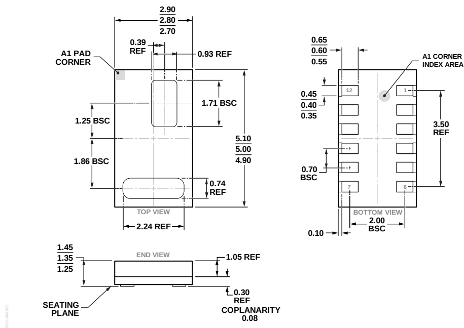
Figure 24. 12-Terminal Chip Array Small Outline No Lead Cavity [LGA_CAV] 2.8 mm × 5.0 mm Body (CE-12-2) Dimensions shown in millimeters
