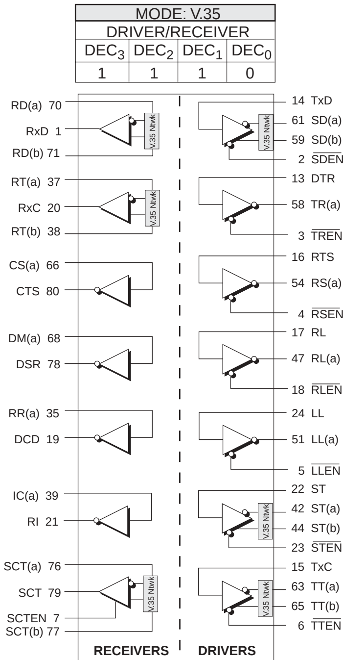
Figure 54. Mode Diagram — V.35
