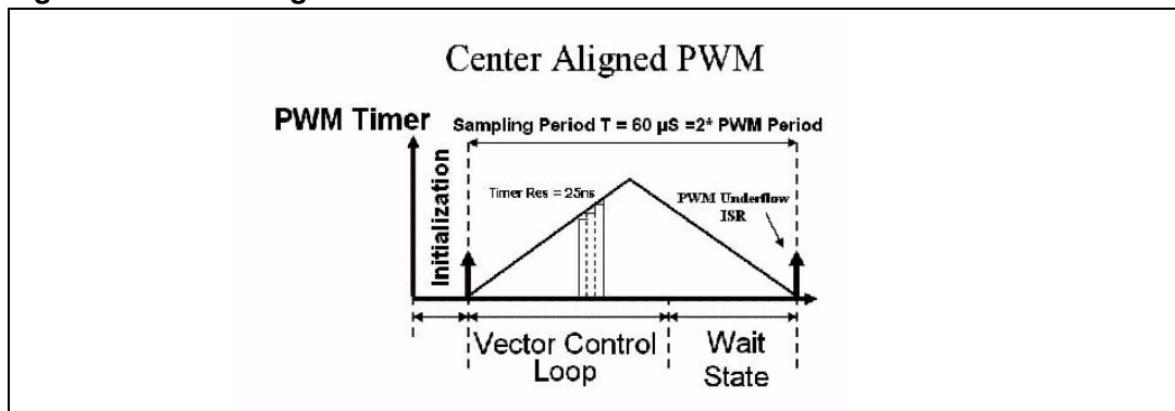
Figure 30. Time diagram
