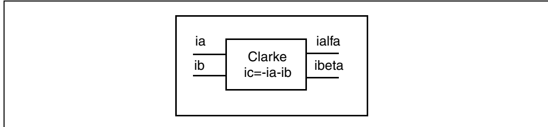
Figure 6. Clark transformation module
