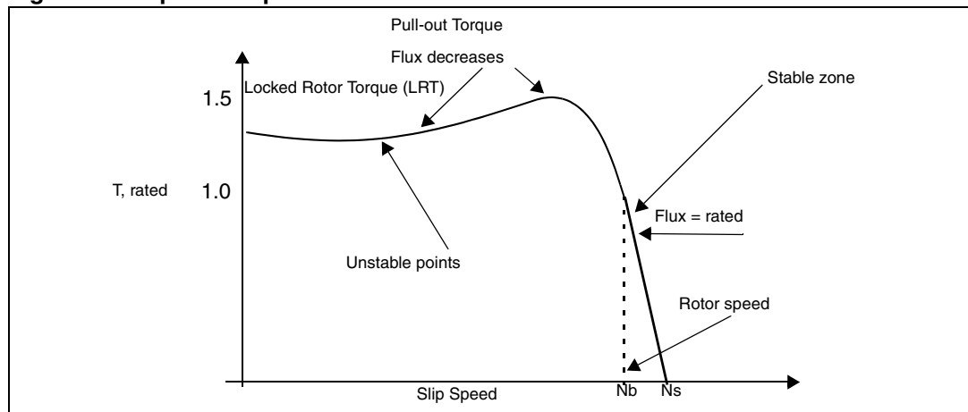
Figure 3. Speed-torque characteristic
