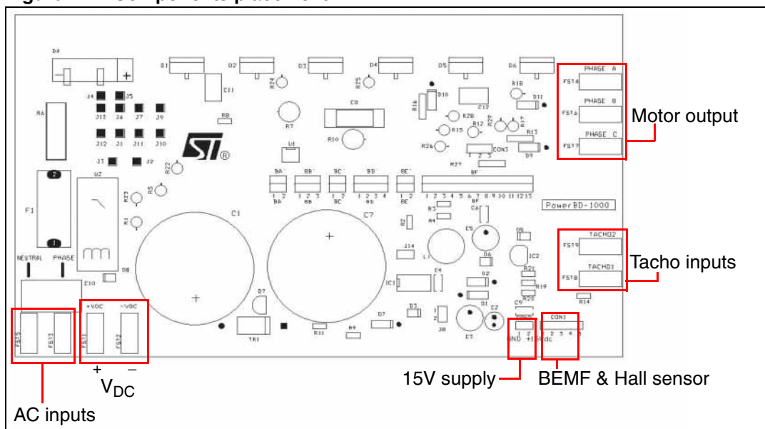
Figure 21. Components placement
