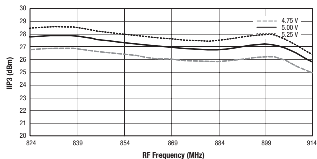
Figure 10. IIP3 vs Frequency and Supply Voltage
