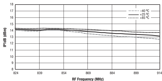
Figure 12. IP1dB vs Frequency and Temperature
