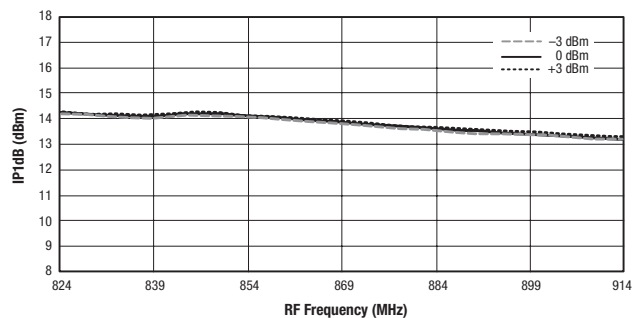
Figure 14. IP1dB vs Frequency and LO Power
