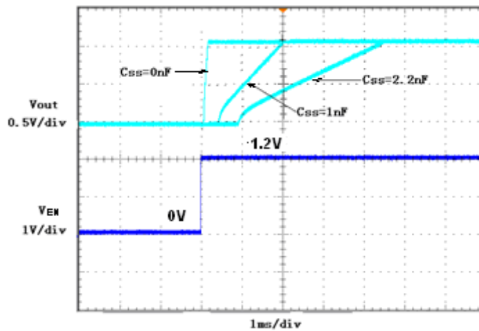
Figure 2. Turn-On Response
