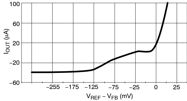
Figure 24. Error Amplifier I OUT vs. V FB (CS5171/3 only)
