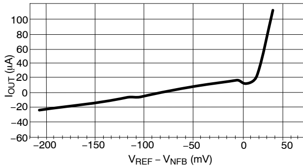
Figure 25. Error Amplifier I OUT vs. V NFB (CS5172/4 only)
