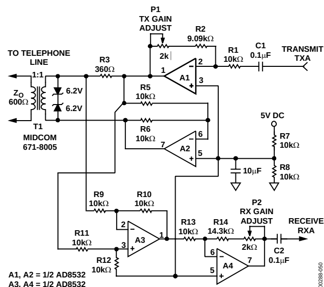
Figure 50. Single-Supply Direct Access Arrangement for Modems
