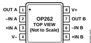
Figure 4. 8-Lead TSSOP (RU Suffix)
