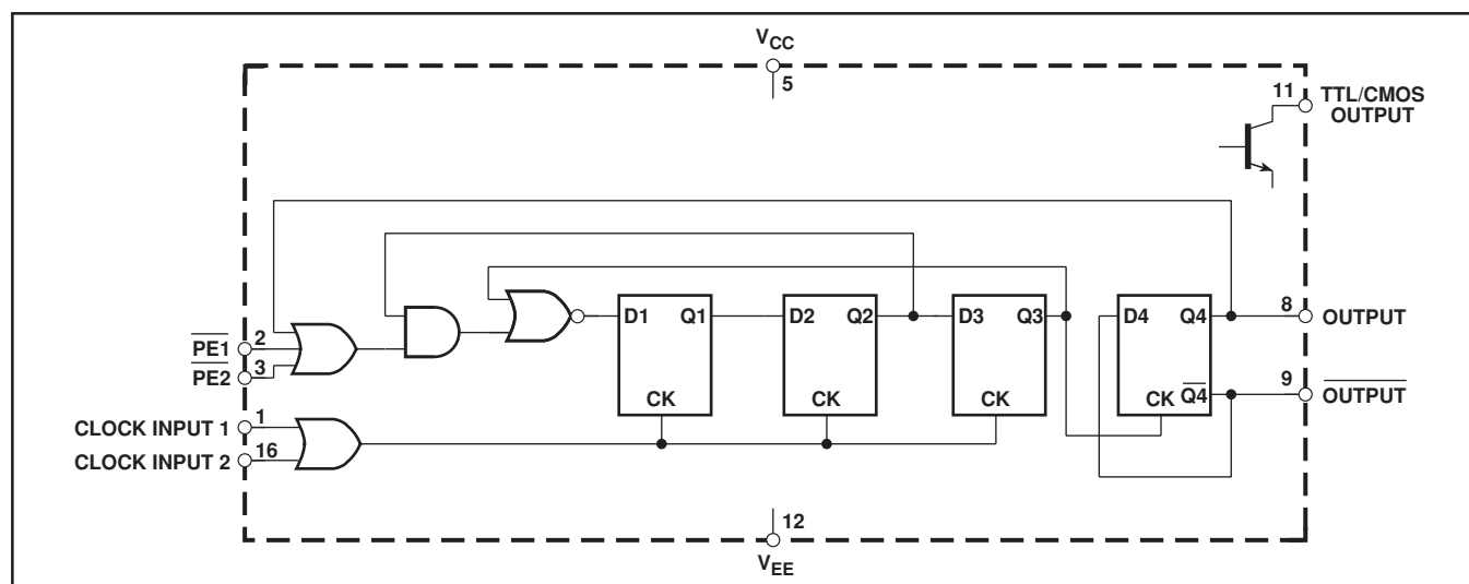
Fig. 2 Functional diagram
