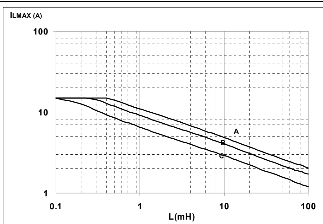
Figure 26. SO-8 maximum turn-off current versus inductance
