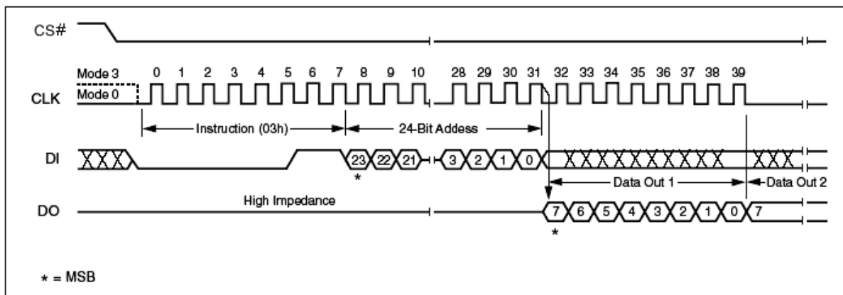
Figure 10. Read Data Instruction Sequence Diagram
