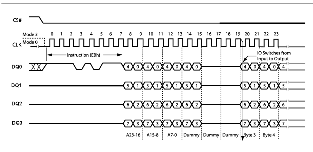
Figure 14. Quad Input / Output Fast Read Instruction Sequence Diagram
