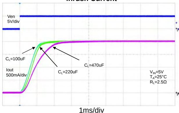
Inrush Current
