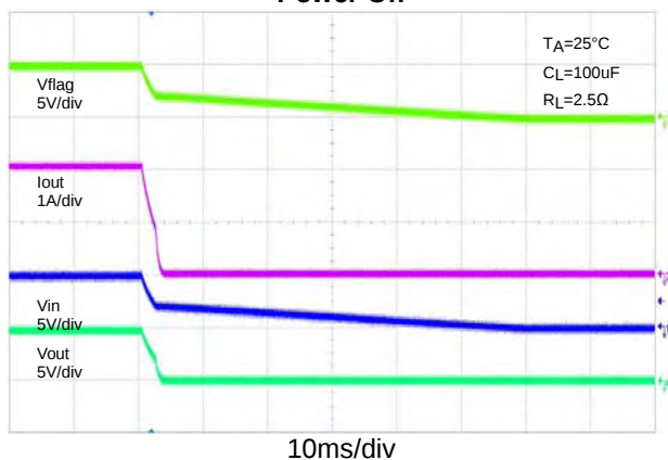
Power Off
