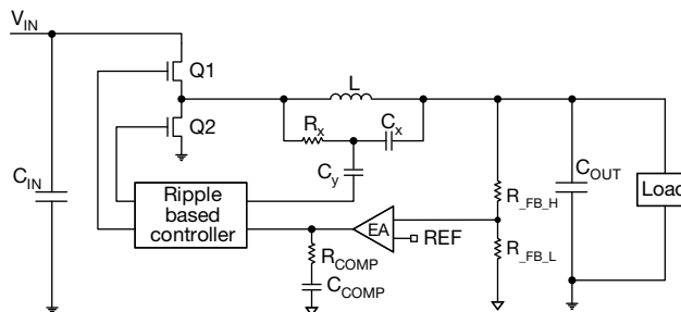
Fig. 6 - SiC47x Control Block Diagram
