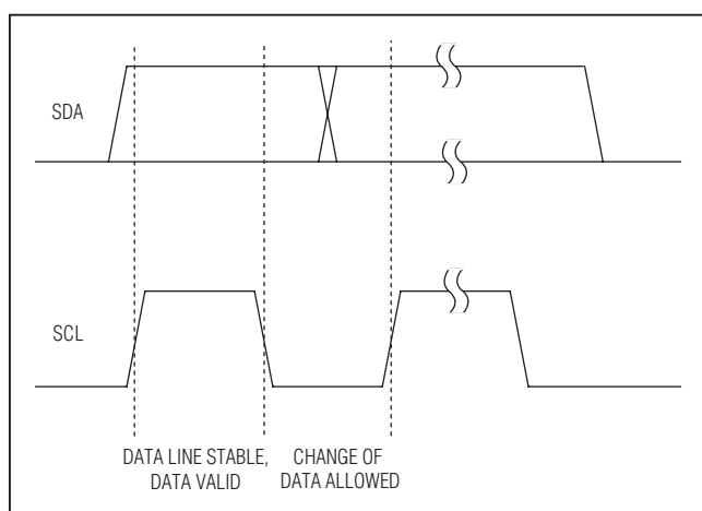
Figure 5. Bit Transfer
