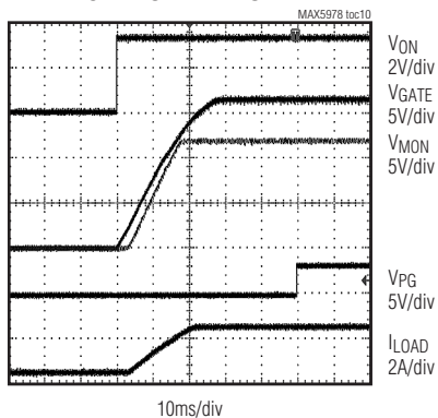
STARTUP WAVEFORM
