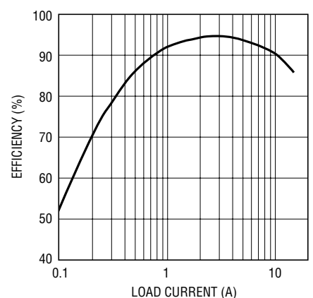
LTC1649 Efficiency
