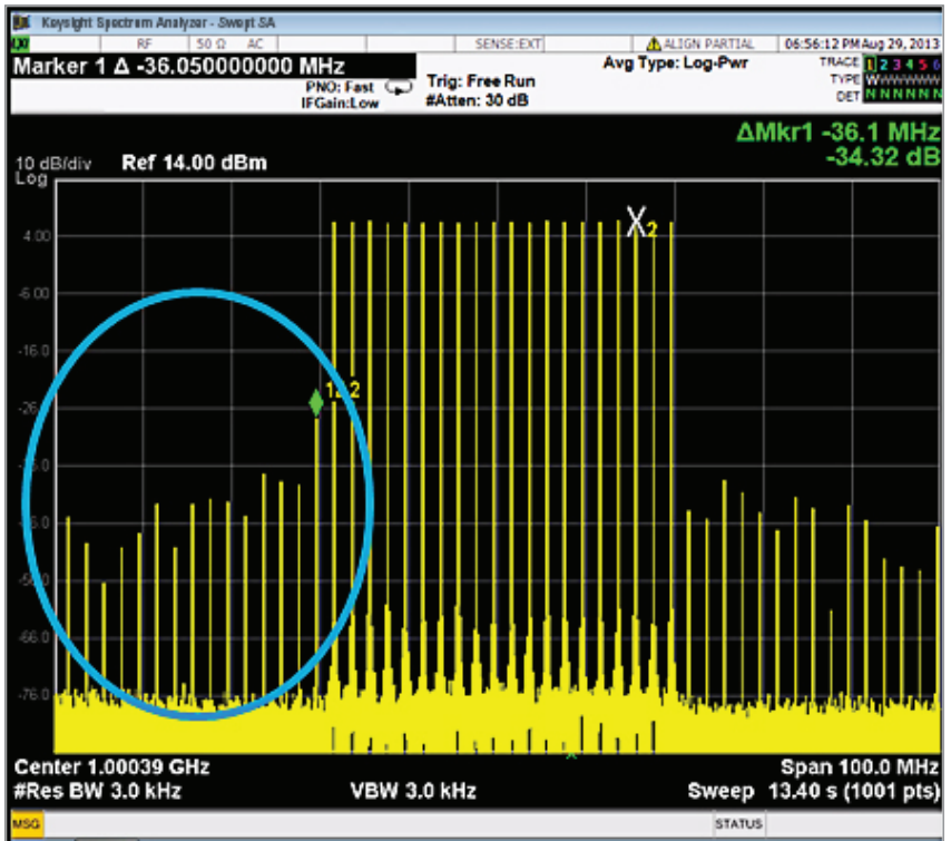
Figure 5. Greater than 15 dBm multi-tone signal without corrections. Distortion products at approximately -34 dBc.
