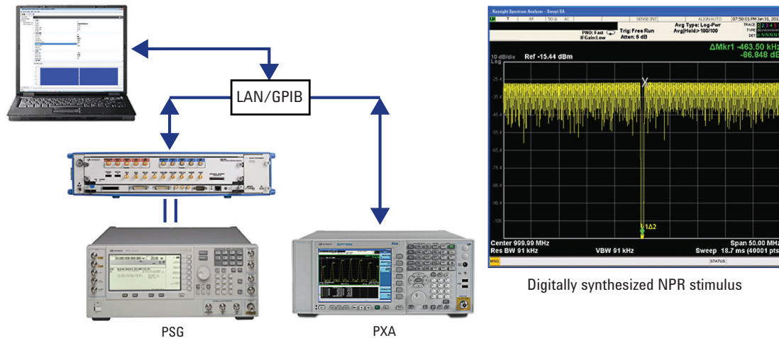
Figure 2. Create specified wideband NPR signals with very sharp and deep notches.
