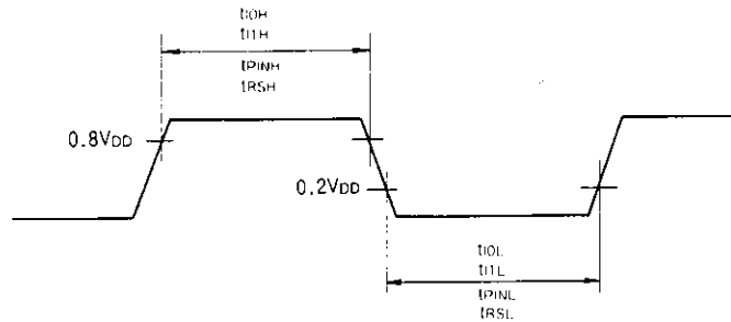
Figure 6: INT0, \overline{INT1} , \overline{INT2} , \overline{INT3} , \overline{INT4} , INT5, PIN1, and \overline{RES} Input Timing
