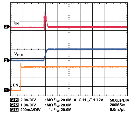
Figure 62. LDO1, LDO2 Startup, V_{OUT} = 1.2 V, I_{OUT} = 5 mA
