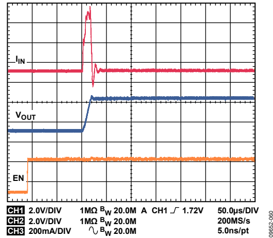
Figure 60. LDO1, LDO2 Startup, V_{OUT} = 3.3 V, I_{OUT} = 5 mA
