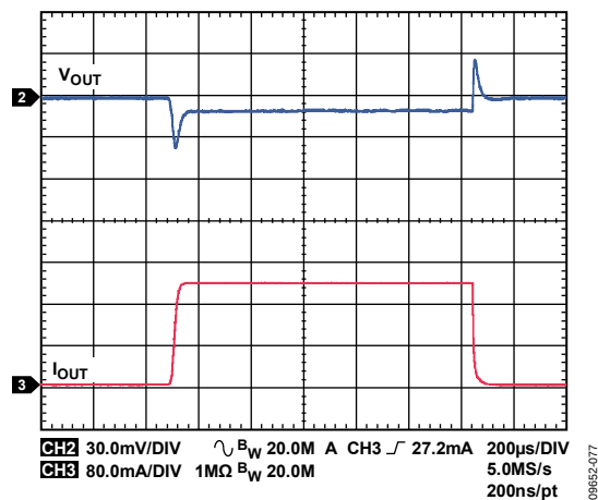
Figure 77. LDO1, LDO2 Response to Load Transient, I_{OUT} from 10 mA to 200 mA, V_{OUT} = 4.7\text{ V}
