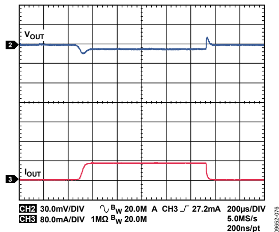
Figure 76. LDO1, LDO2 Response to Load Transient, I_{OUT} from 1 mA to 80 mA, V_{OUT} = 4.7\text{ V}
