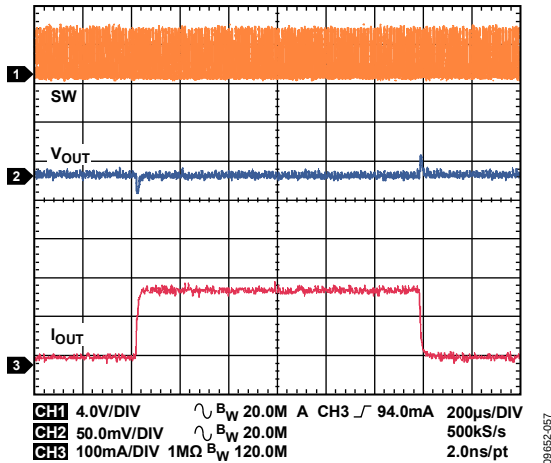
Figure 57. Buck Response to Load Transient, I_{OUT1} = 20 mA to 200 mA, V_{OUT1} = 1.2 V, PWM Mode
