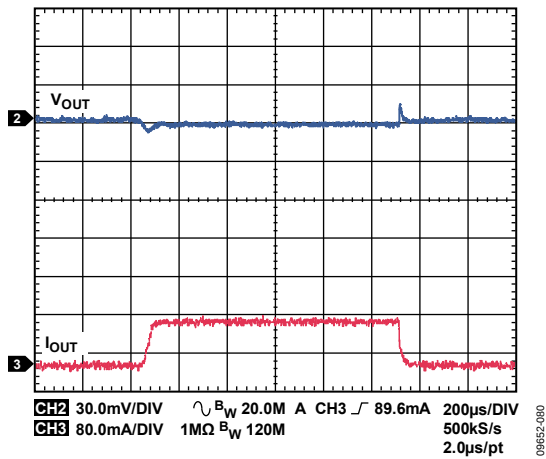
Figure 80. LDO1, LDO2 Response to Load Transient, I_{OUT} from 1 mA to 80 mA, V_{OUT} = 1.8\text{ V}
