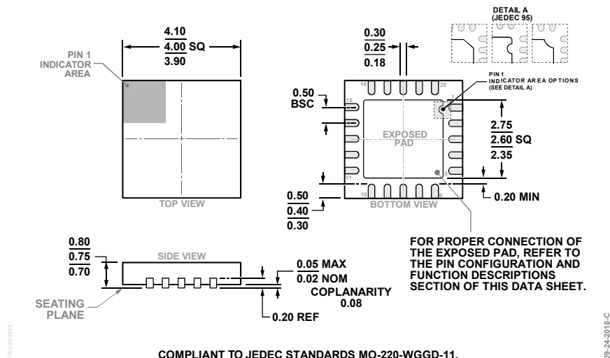
Figure 115. 20-Lead Lead Frame Chip Scale Package [LFCSP] 4 mm × 4 mm Body and 0.75 mm Package Height (CP-20-8)
