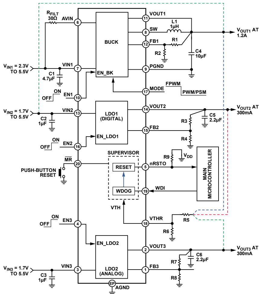
Figure 113. Application Diagram
