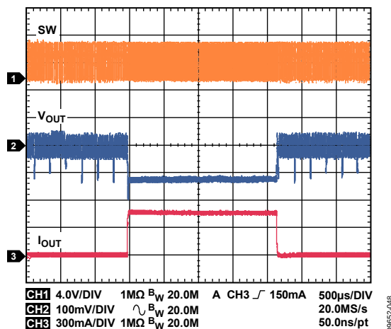
Figure 48. Buck Response to Load Transient, I_{OUT1} = 50 mA to 500 mA, V_{OUT1} = 3.3 V, Auto Mode
