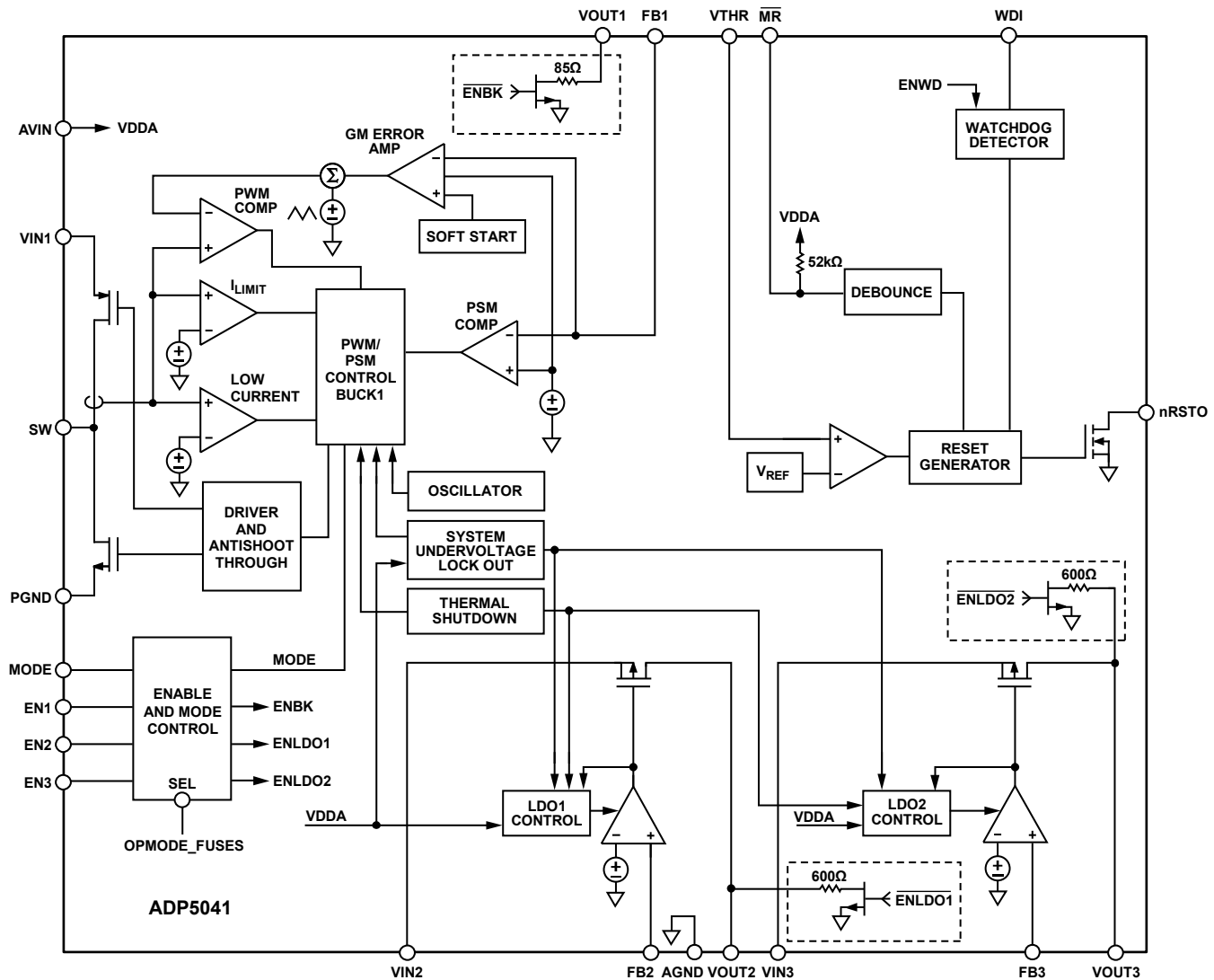
Figure 101. Functional Block Diagram
