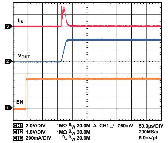
Figure 61. LDO1, LDO2 Startup, V_{OUT} = 1.8 V, I_{OUT} = 5 mA
