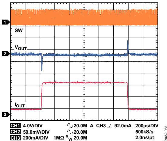
Figure 58. Buck Response to Load Transient, I_{OUT1} = 50 mA to 500 mA, V_{OUT1} = 1.2 V, PWM Mode
