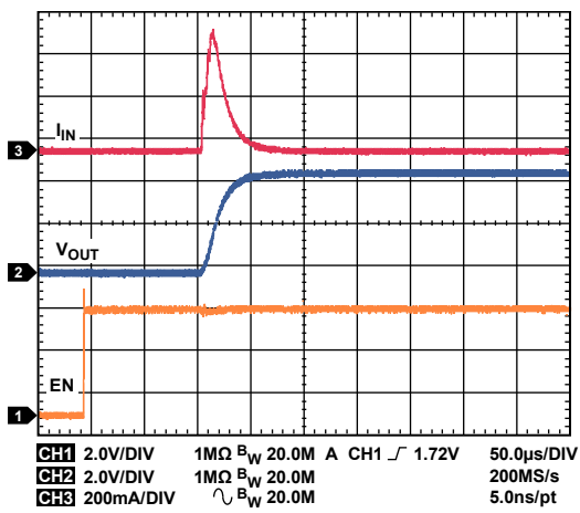
Figure 59. LDO1, LDO2 Startup, V_{OUT} = 4.7 V, I_{OUT} = 5 mA
