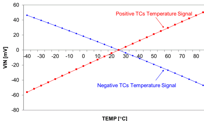
Figure 14. Temperature signals of positive and negative TC bridge resistance sensors
