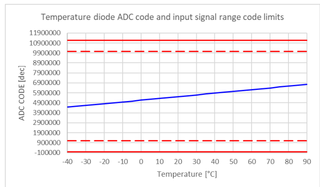
Figure 12b. ADC output code [dec]
