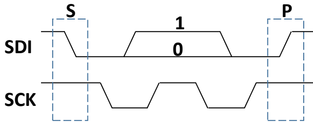
Figure 7. I2C bus protocol definitions
