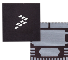
FK Suffix (Pb-Free) 24 PIN PQFN 98ASA00428D
