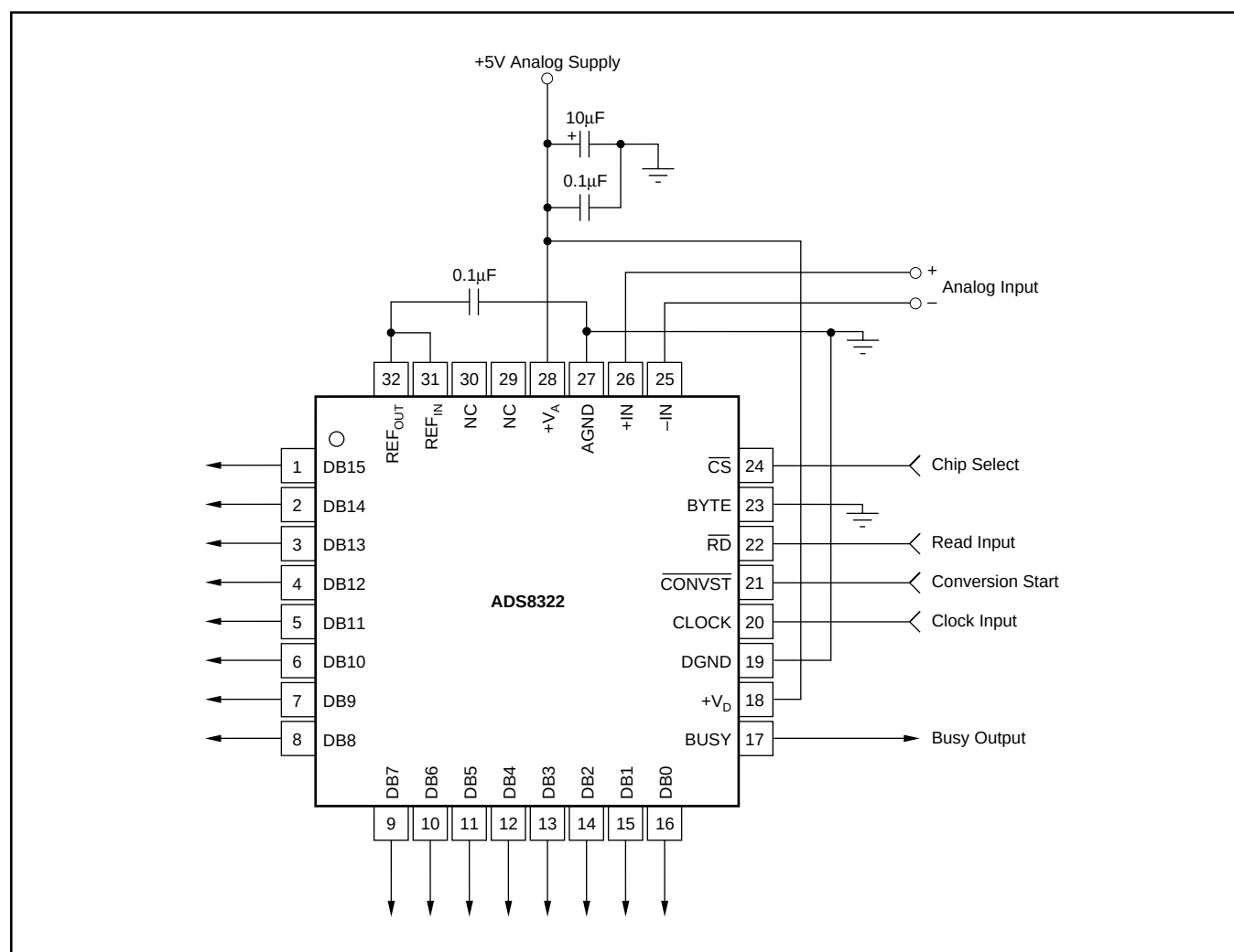
FIGURE 1. Typical Circuit Configuration.
