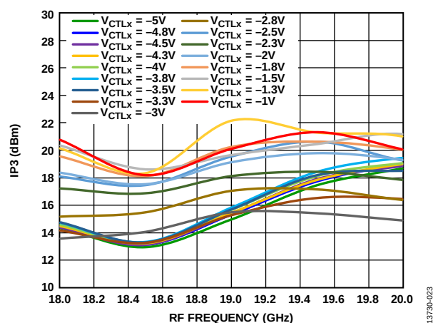
Figure 23. Input IP3 vs. RF Frequency at Various Control Voltages, LO = 4 dBm
