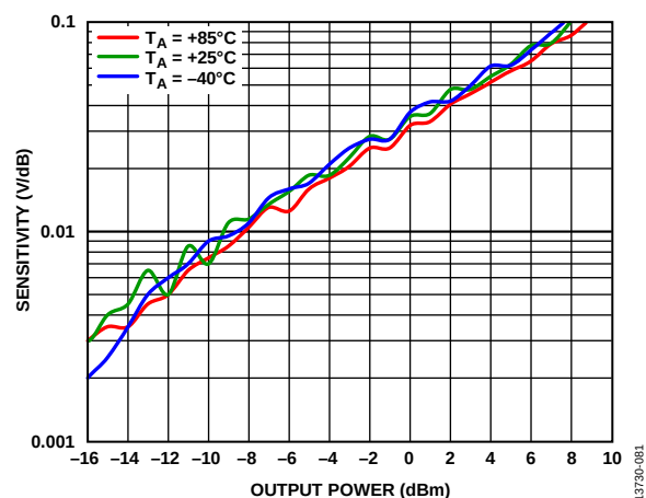
Figure 81. Detector Sensitivity vs. Output Power at Various Temperatures, LO = 23.5 GHz
