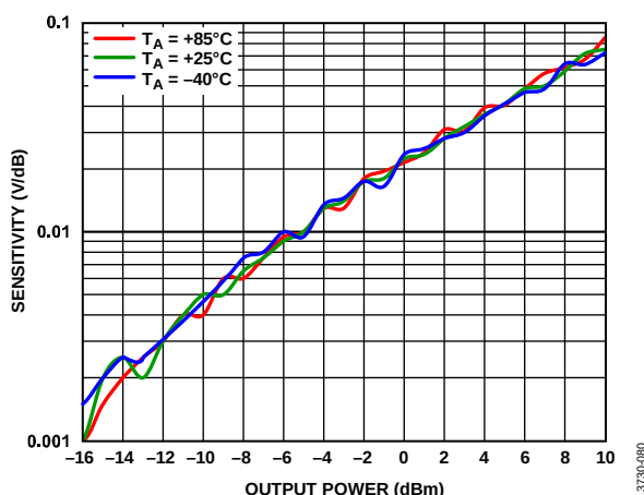
Figure 80. Detector Sensitivity vs. Output Power at Various Temperatures, LO = 22 GHz
