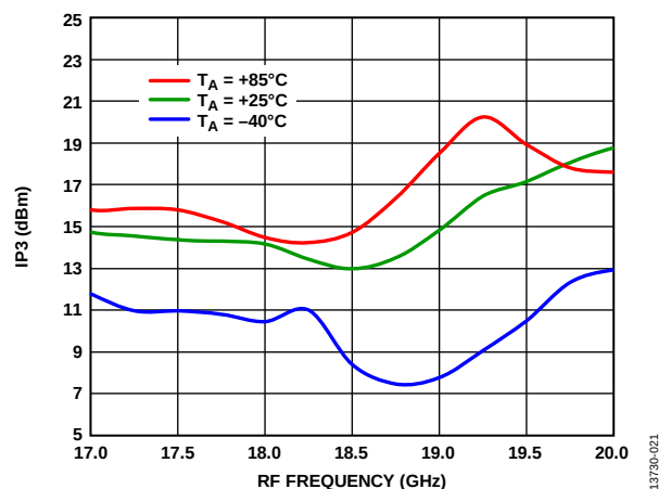
Figure 21. Input IP3 vs. RF Frequency at Various Temperatures, LO = 4 dBm
