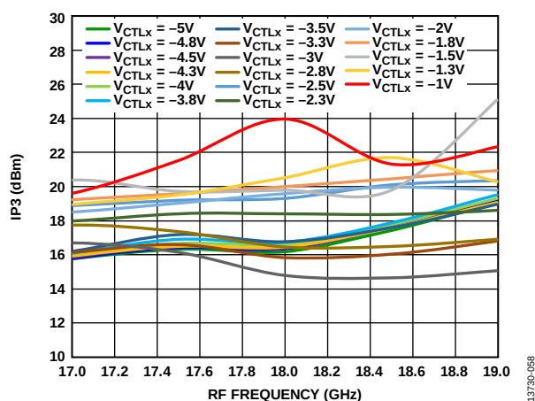
Figure 58. Input IP3 vs. RF Frequency at Various Control Voltages, LO = 4 dBm
