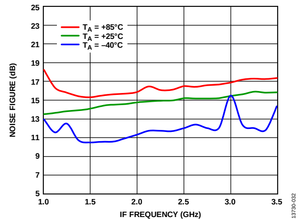
Figure 32. Noise Figure vs. IF Frequency at Various Temperatures, LO = 6 dBm, LO Frequency = 21 GHz
