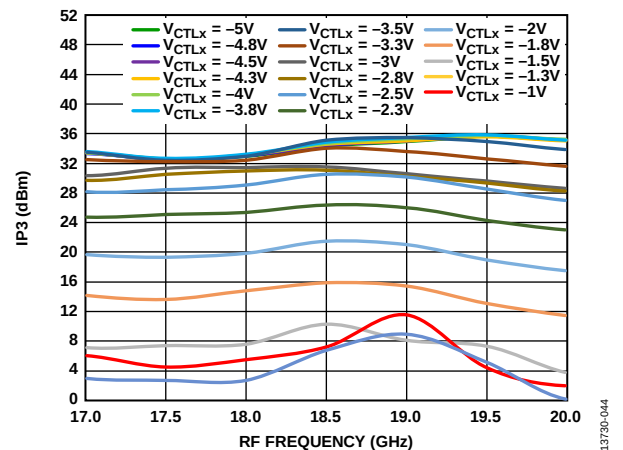
Figure 44. Output IP3 vs. RF Frequency at Various Control Voltages, LO = 4 dBm
