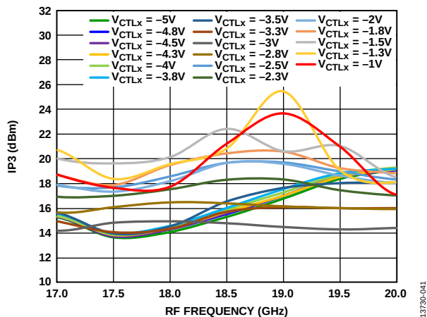
Figure 41. Input IP3 vs. RF Frequency at Various Control Voltages, LO = 4 dBm
