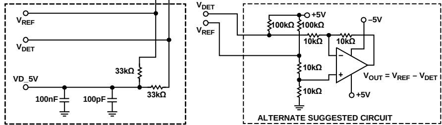
Figure 83. Typical Application Circuit
