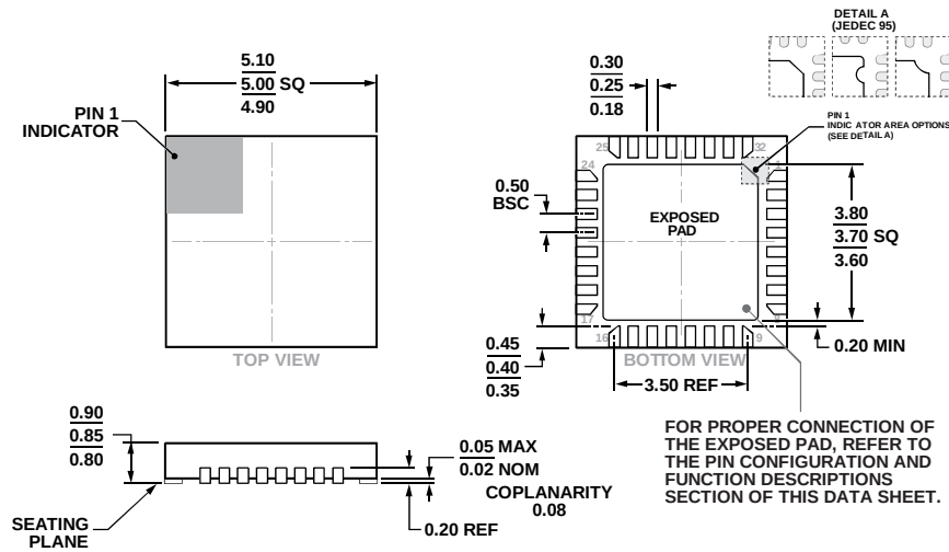
Figure 85. 32-Lead Lead Frame Chip Scale Package [LFCSP] 5 mm x 5 mm Body and 0.85mm Package Height (HCP-32-1)
