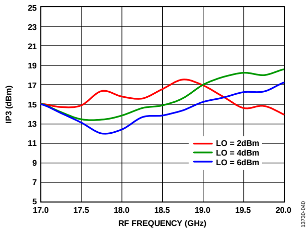
Figure 40. Input IP3 vs. RF Frequency at Various LO Powers
