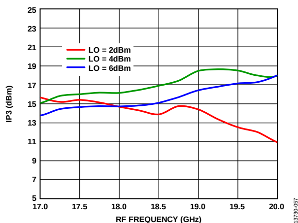
Figure 57. Input IP3 vs. RF Frequency at Various LO Powers
