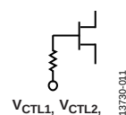
Figure 11. V_{CTL1} , V_{CTL2} Interface
