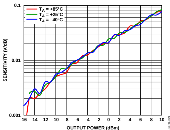
Figure 79. Detector Sensitivity vs. Output Power at Various Temperatures, LO = 20.5 GHz
