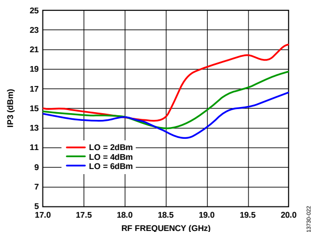
Figure 22. Input IP3 vs. RF Frequency at Various LO Powers
