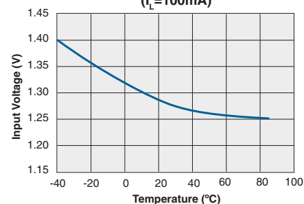
CPC1218 Typical Input Voltage for Switch Operation vs. Temperature (I_L = 100\text{mA})
