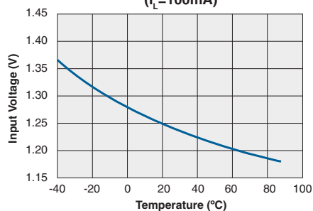
CPC1218 Typical Input Voltage for Switch Dropout vs. Temperature (I_L = 100\text{mA})
