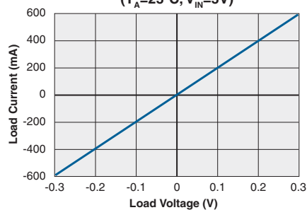
CPC1218 Typical Load Current vs. Load Voltage (T_A = 25^\circ\text{C}, V_{IN} = 5\text{V})
