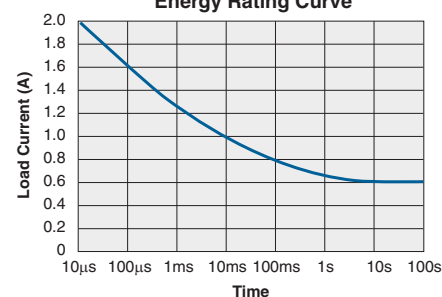
CPC1218 Energy Rating Curve
