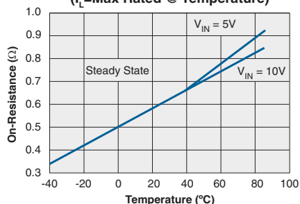
CPC1218 Typical On-Resistance vs. Temperature (I_L = \text{Max Rated @ Temperature})
