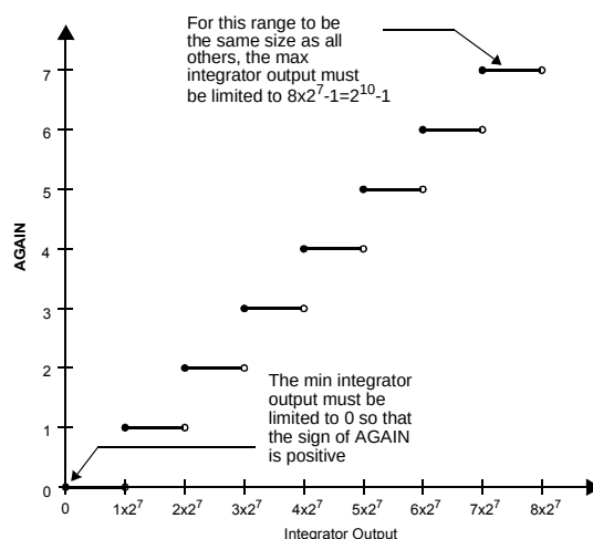
Figure 38. AGC integrator output limits
