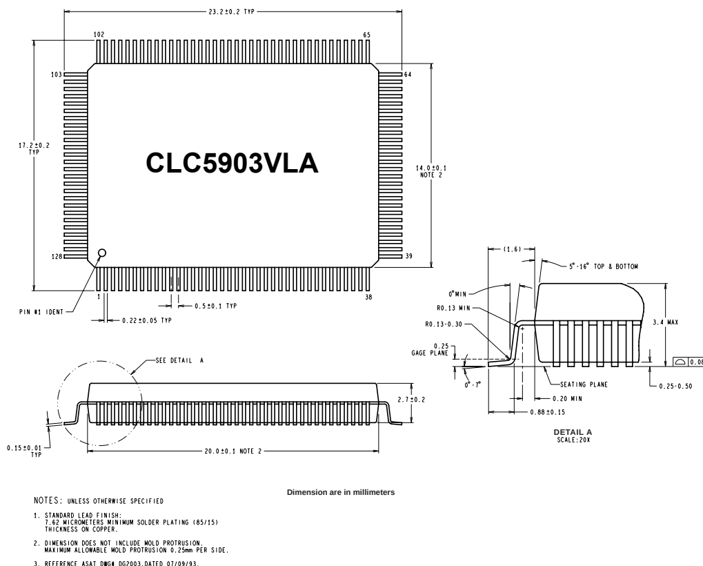
Figure 40. CLC5903VLA PQFP Package Dimensions
