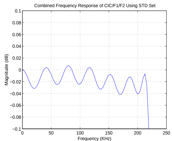
Figure 26. CIC, F1, & F2 STD Passband Flatness
