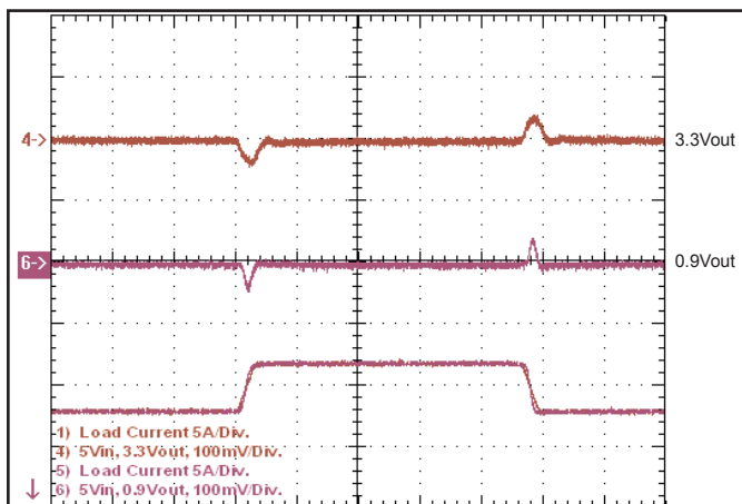
Figure 17: Output voltage response at 5.0Vin to step-change in load current (50-75-50% of Iout max; di/dt=0.1A/μs). Load cap: 15μF, 100mΩ ESR tantalum and 10μF ceramic. Top: Vout (100mV/div), Bottom: Iout (5A/div).
