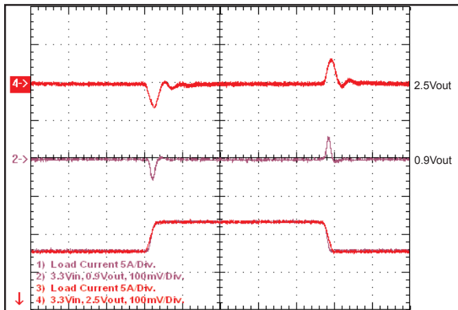
Figure 15: Output voltage response at 3.3Vin to step-change in load current (50-75-50% of Iout max; di/dt=0.1A/μs). Load cap: 15μF, 100mΩ ESR tantalum and 10μF ceramic. Top: Vout (100mV/div), Bottom: Iout (5A/div).
