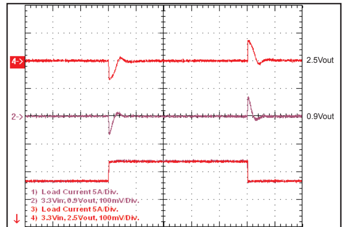
Figure 16: Output voltage response at 3.3Vin to step-change in load current (50-75-50% of Iout max; di/dt=3A/μs). Load cap: 470μF, 25mΩ ESR tantalum and 10μF ceramic. Top: Vout (100mV/div), Bottom: Iout (5A/div).
