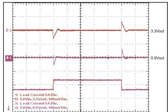
Figure 18: Output voltage response at 5.0Vin to step-change in load current (50-75-50% of Iout max; di/dt=3A/μs). Load cap: 470μF, 25mΩ ESR tantalum and 10μF ceramic. Top: Vout (100mV/div), Bottom: Iout (5A/div).
