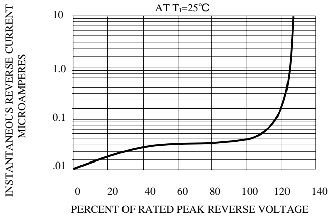
FIG. 4-TYPICAL REVERSE CHARACTERISTICS AT T J =25°C
