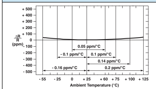
FIGURE 3 - TYPICAL TCR CURVE Z-FOIL
