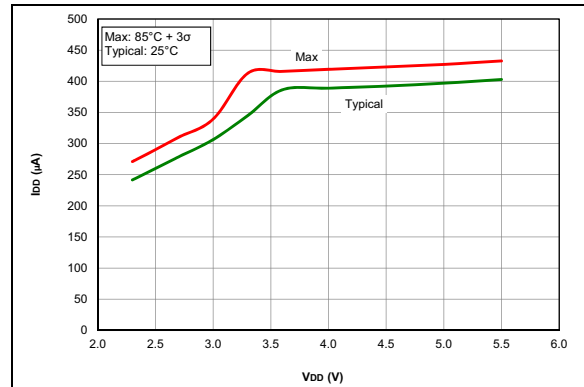
FIGURE 38-56: I_{DD} , XT Oscillator 4 MHz, PIC16LF15356/75/76/85/86 devices only
