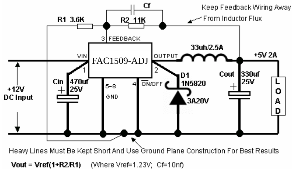
Figure 3. Typical Application of FAC1509
