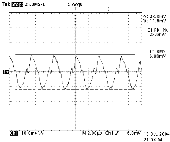
Figure 11: Output ripple & noise at 12Vin, 6.5V/3A out
