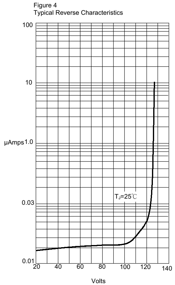
Instantaneous Reverse Current - MicroAmperes versus Percent of Rated Peak Reverse Voltage - Volts
