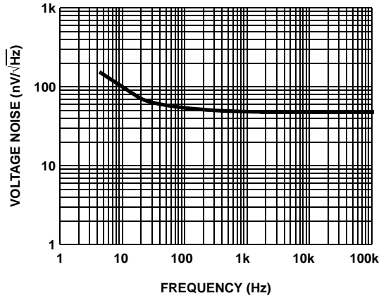
FIGURE 12. VOLTAGE NOISE vs FREQUENCY
