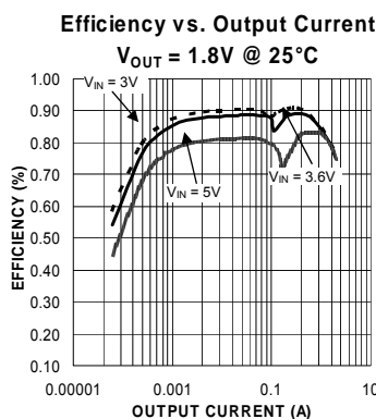
Figure 2. Efficiency Under Load
