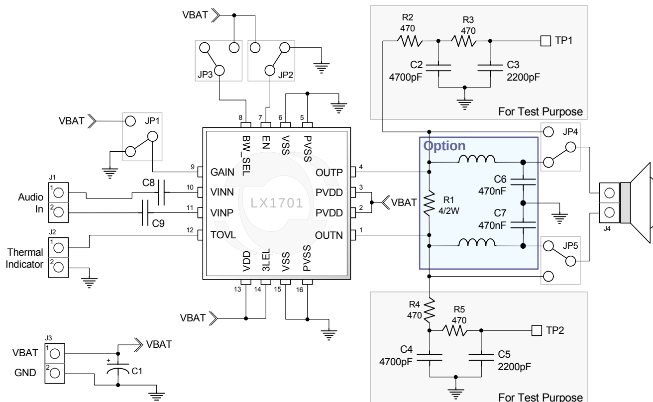
Figure 4 – LXE1701 Evaluation Module Schematic
