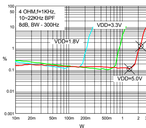
THD+N vs. Power
