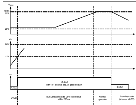
Figure 3 State of Operation respect to VCC
