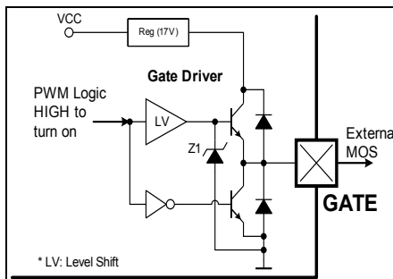
Figure 13 Gate Driver
