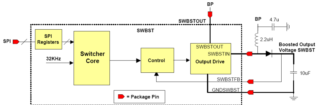
Figure 23. Boost Switcher Architecture
