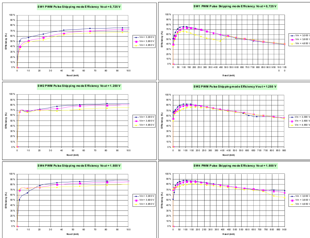
Figure 19. Buck Switcher PWM (Pulse Skipping) Efficiency
