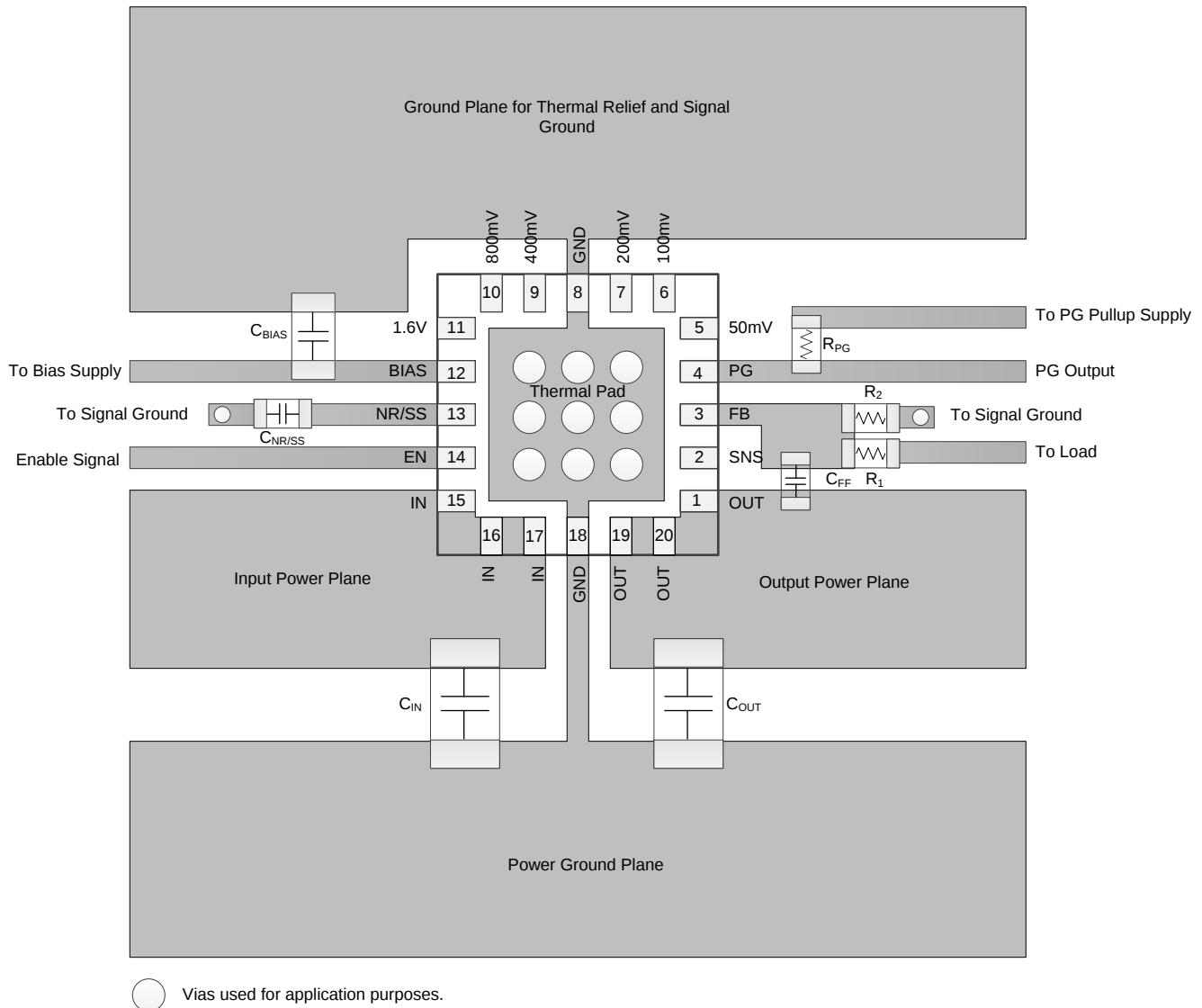
Figure 73. Example Layout
