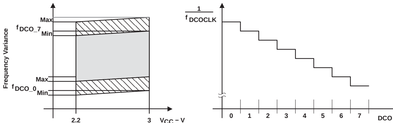
Figure 12. DCO Characteristics
