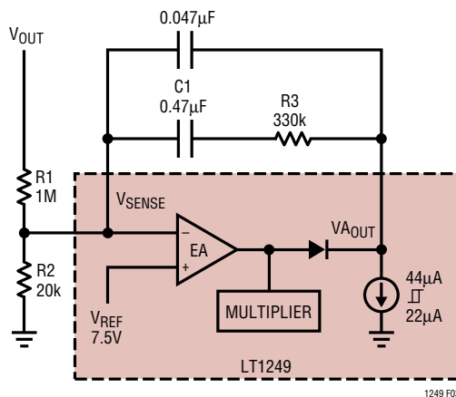
Figure 3. Overvoltage Protection
